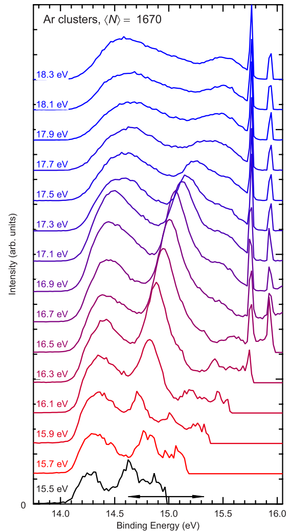
FIG. 1. (Color online) High-resolution 3p (valence band) photoelectron spectra of Ar clusters at photon energies from 15.5 to 18.3 eV. The mean cluster size (from the scaling laws) is \langle N \rangle = 1670 . Data recorded with the Scienta analyzer. The sharp, spin-orbit split atomic lines at 15.76 and 15.94 eV binding energy are below the usable energy range of the analyzer at h\nu = 16.1 eV. A horizontal arrow marks the extent of the observed dispersion.
