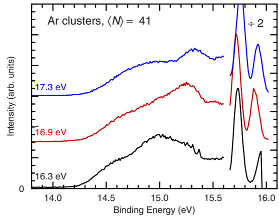
FIG. 3. (Color online) Low-resolution 3p (valence-band) photoelectron spectra of Ar clusters at different photon energies recorded with the magnetic bottle analyzer. The mean cluster size is \langle N \rangle = 41 .
