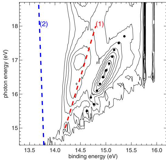
FIG. 2. (Color online) Contour plot showing high-resolution 3p photoelectron spectra of Ar clusters with mean size \langle N \rangle = 1670 as a function of both photon energy and binding energy. The peak maxima of the \approx 15 eV feature showing dispersion are indicated by black dots. High-resolution data recorded with the Scienta analyzer. The lines designated 1 and 2 derive from the photoemission data for Ar(111) measured by Kassühlke et al. (Ref. 18). See text.
